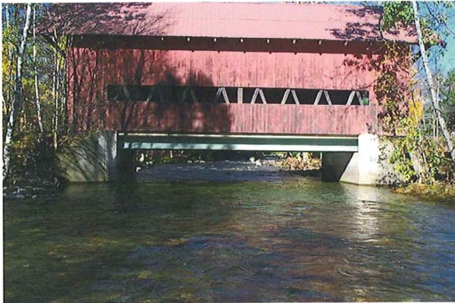
Figure 15. Undersized Brook Road Bridge
