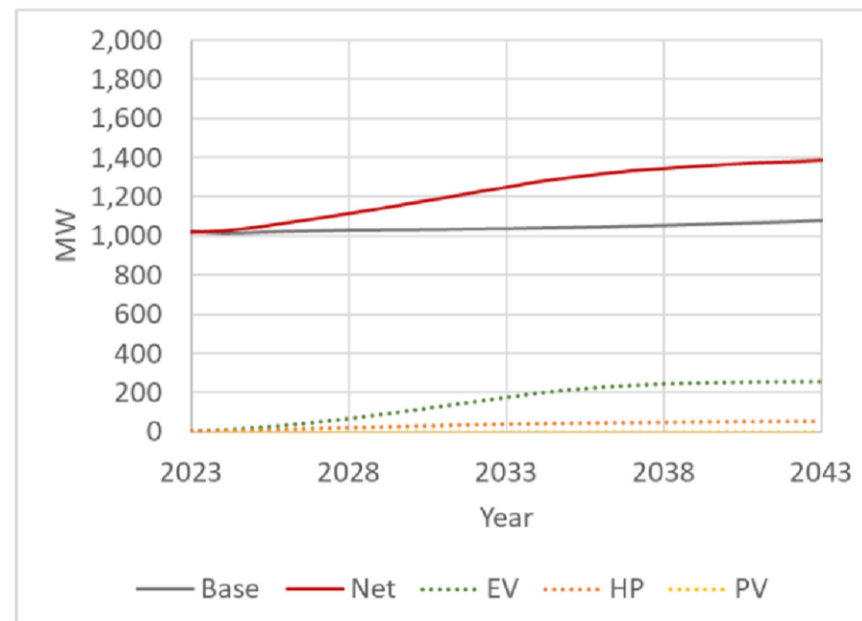
Figure 5: Projected Vermont Summer Peak Load and Its Component Forecasts Source: VELCO 2024 Long-Range Transmission Plan
