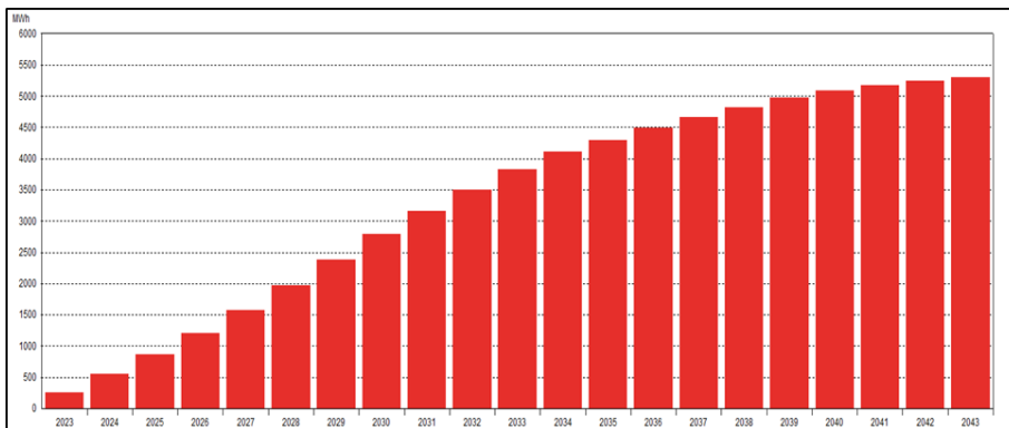
Figure 6: Heat Pump Loads 2043 Source: Stowe Electric Department, 2024
